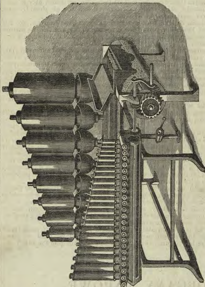
Organy parowe.
